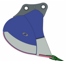
PROFIL 40T STD/R* koparki 39-47t lemesz 440x60mm
